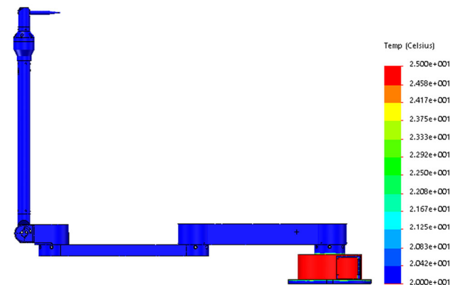
Fig. 23 Thermal distribution analysis of PCMA
