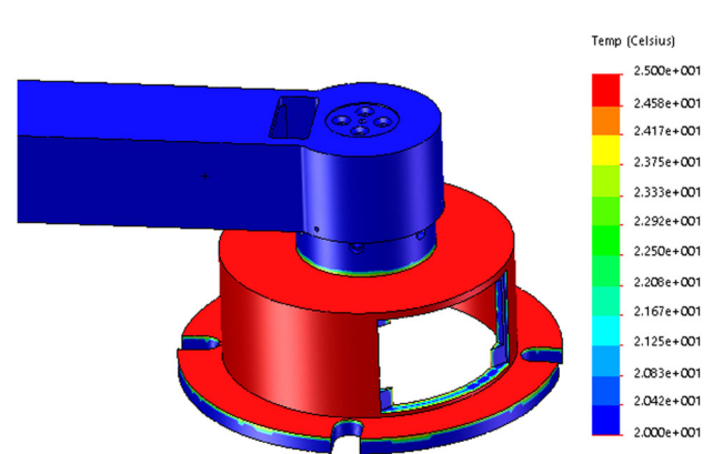
Fig. 24 Thermal distribution around base frame
