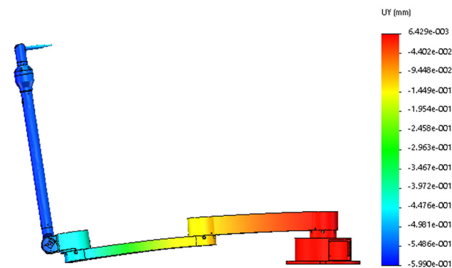
Fig. 22 Static deformation by self-weight of PCMA
